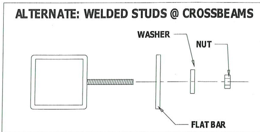
DETAIL: ATTACHMENT OF SOUND CURTAIN TO HORIZONTAL STRUCTURAL STEEL SUPPORTS
